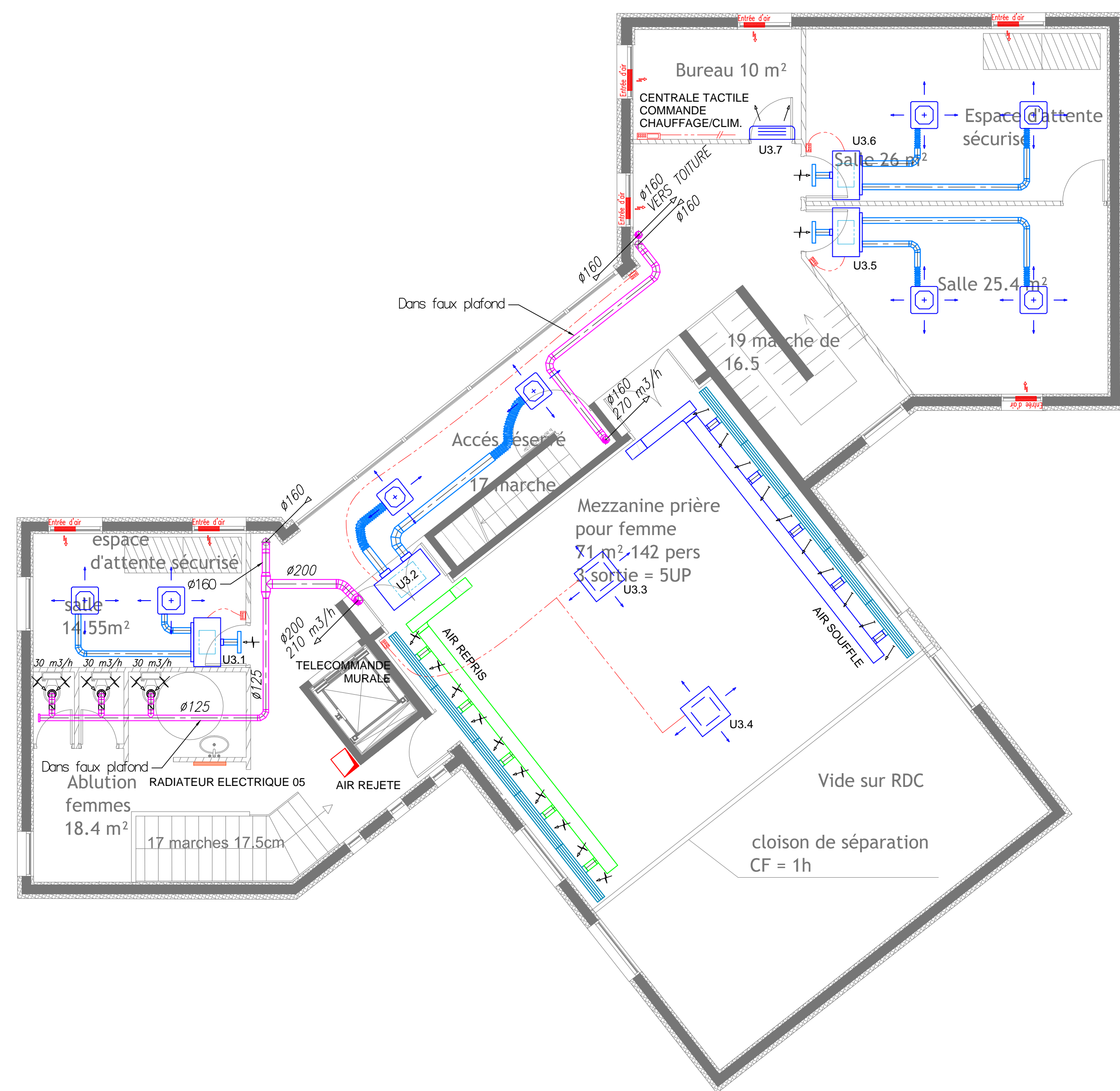
PLAN R+1
